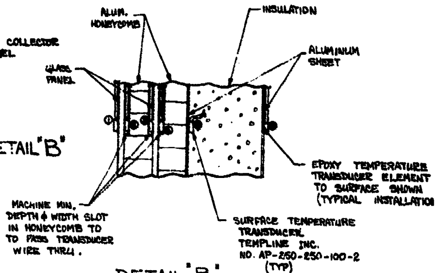
DETAIL "B"
